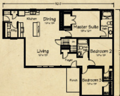
Basement Plan
