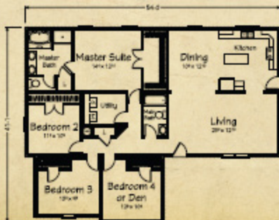
Crawlspace Plan
