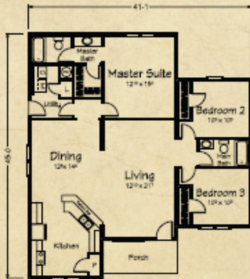
Crawlspace Plan
